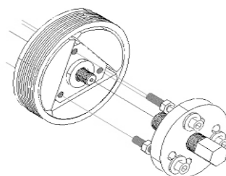
Figure 24 Clutch puller installation
