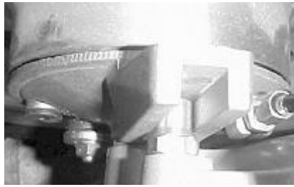
Figure 4, from the brake hub
