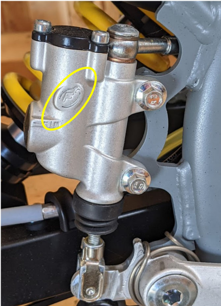
Formula - Rebuild kit BCKG0015 (11.0mm)
